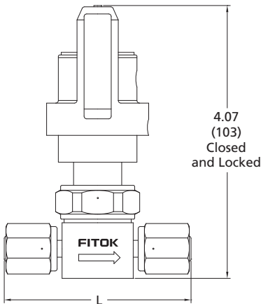
Female FR Fittings
